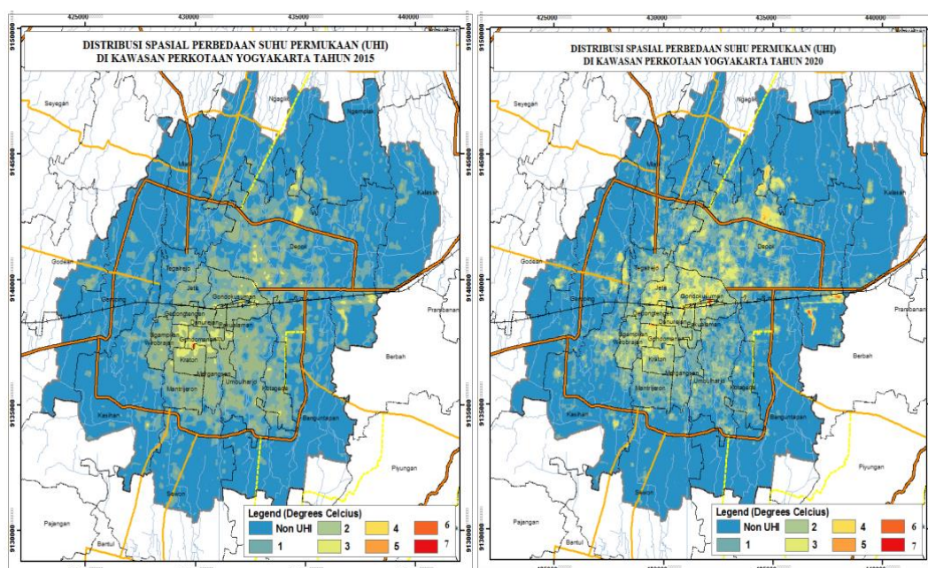
Gambar 2. Dinamika Spasial-Temporal LST
