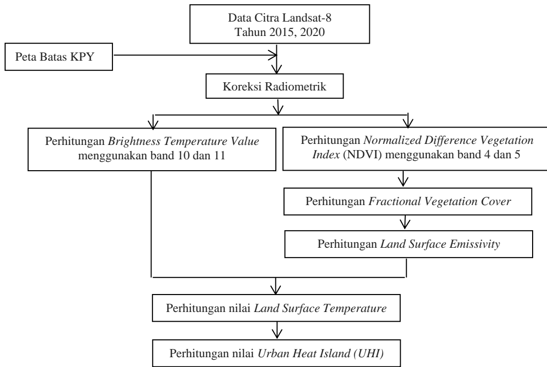
Gambar 2. Alur Analisis Penelitian
