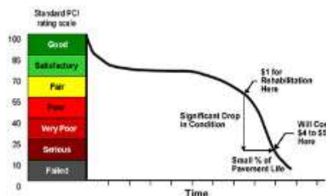
Figure 14. PCI rating vs dan Time (Colorado State University, 2013)
